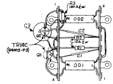
#54A3077 A.C. SOLENOID ASSY. TP2 TP3
