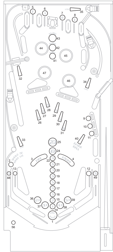
Location of lamps on playfield
