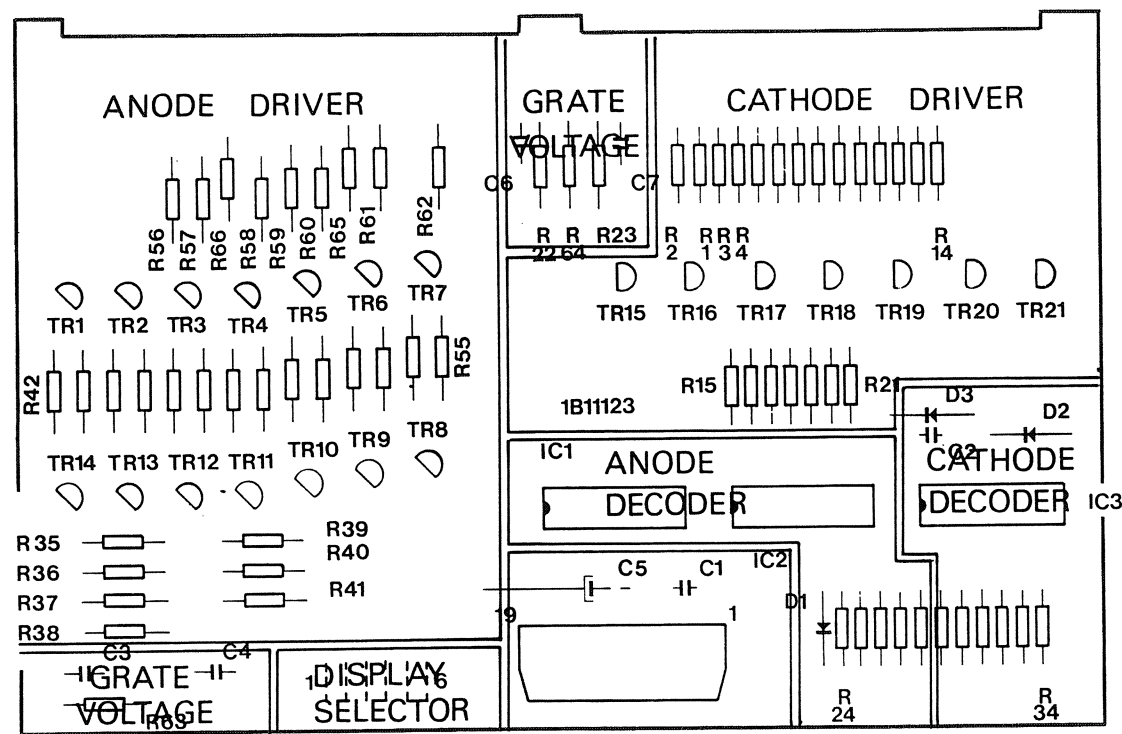
C.P.U. BOARD
